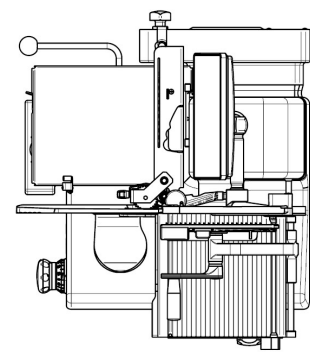
VSP A 10" display top view
